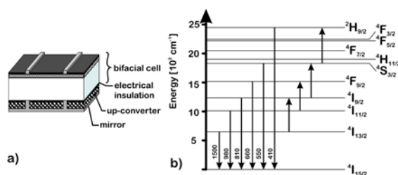
Figure 1: a) Arrangement of an up-converter applied to the rear of a bifacial solar cell, b) energy level diagram of trivalent erbium. The upward arrows indicate possible excitations at about 1500 nm. The emissions as a result of the up-conversion process (downward arrows) are all within the absorption range of silicon.
