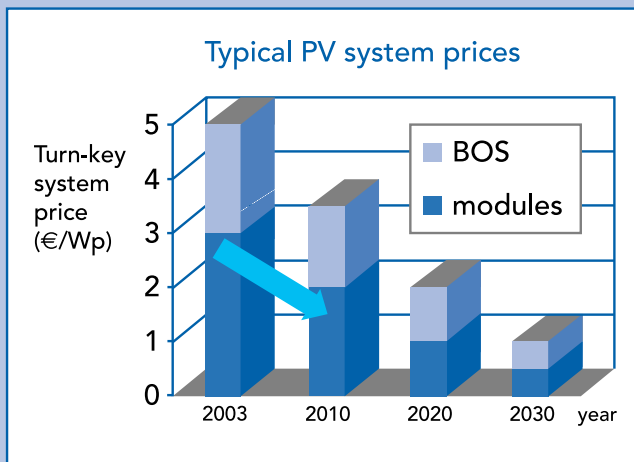
Figure 1. Possible development of turn-key system prices (2), divided into modules and BOS-components.
