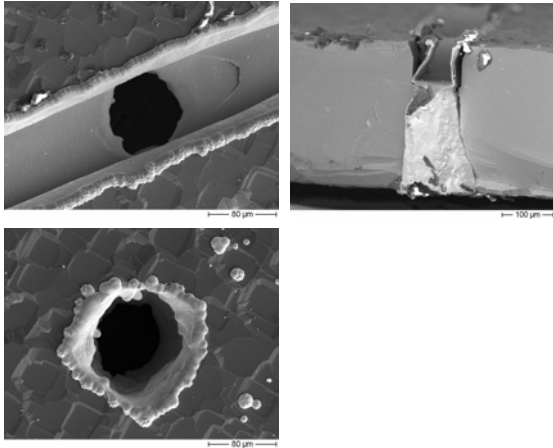
Fig.3 Electron microscopy pictures of the plated grooves and holes
