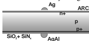
Fig.1 Cross-section of the boron BSF solar cell
