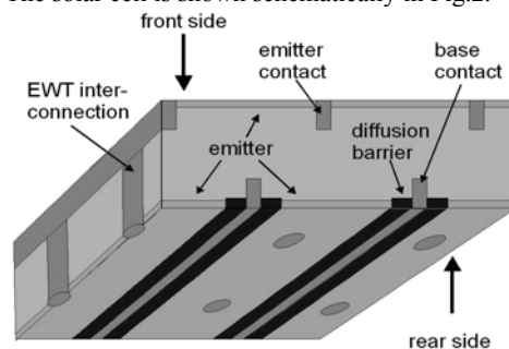
Fig.2 Schematic view of the bifacial solar cell
