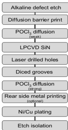
Fig.4 Process sequence of a double sided emitter solar cell
