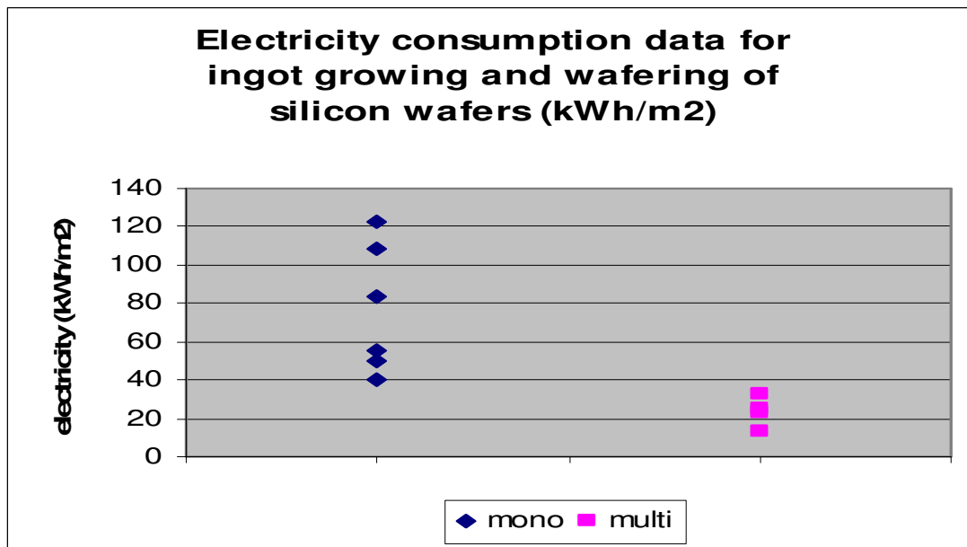
Figure 5: Variation in electricity consumption between different ingot/wafer manufacturers. Wafer thickness 240-270 μm for mono-Si wafers, 200-240 μm for multi-Si.
